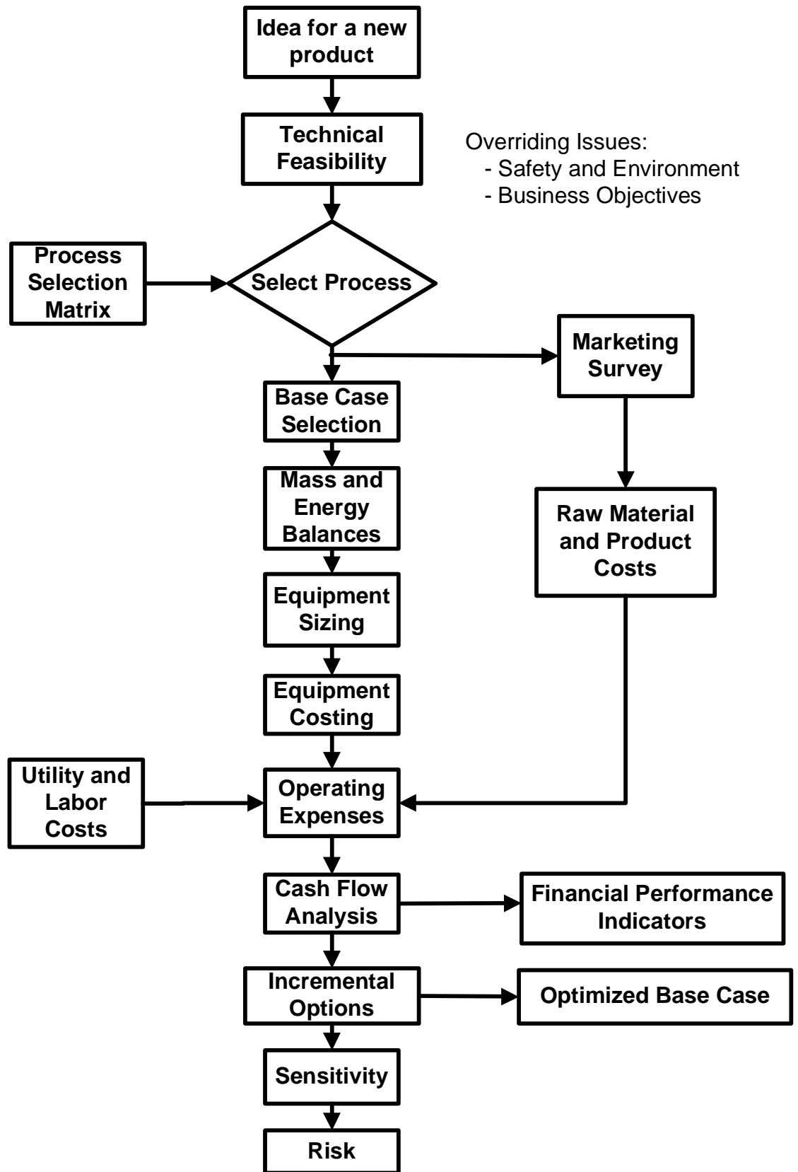
Flowsheet of the Design Case
