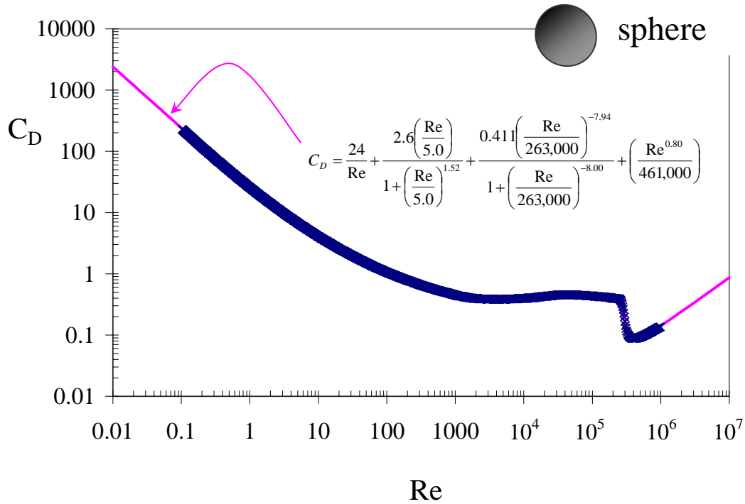
Figure 1: Equation 1 captures drag coefficient as a function of Reynolds number over the entire Reynolds-number range of the available experimental data. Also shown are data for uniform flow around a sphere (Schlichting, 1955). Use beyond Re=10^6 is not recommended; for Re<2 equation 1 follows the creeping-flow result ( C_D=24/Re ).
